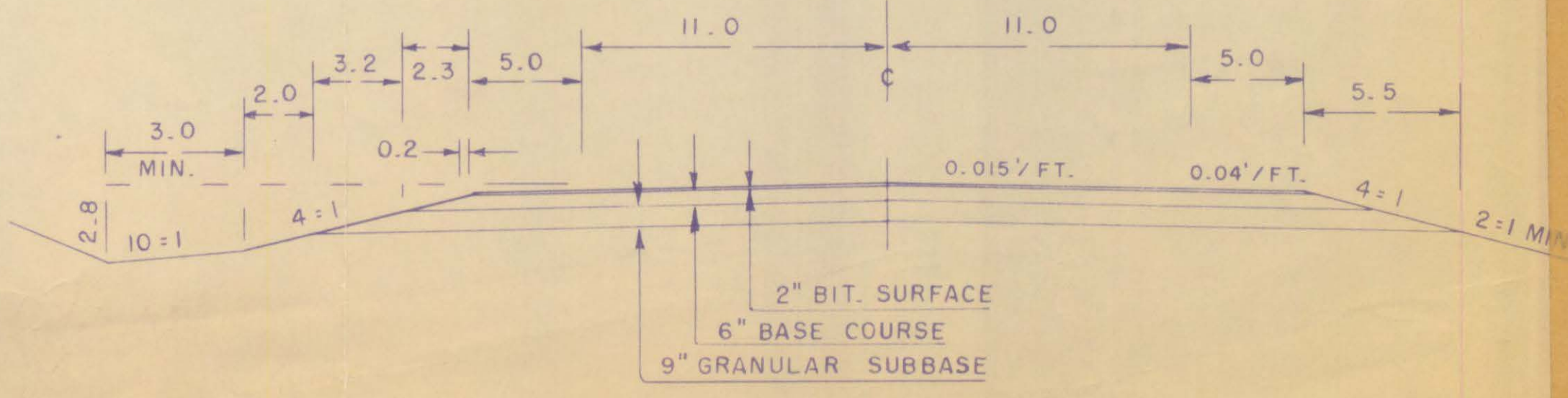
TYPICAL SECTION
