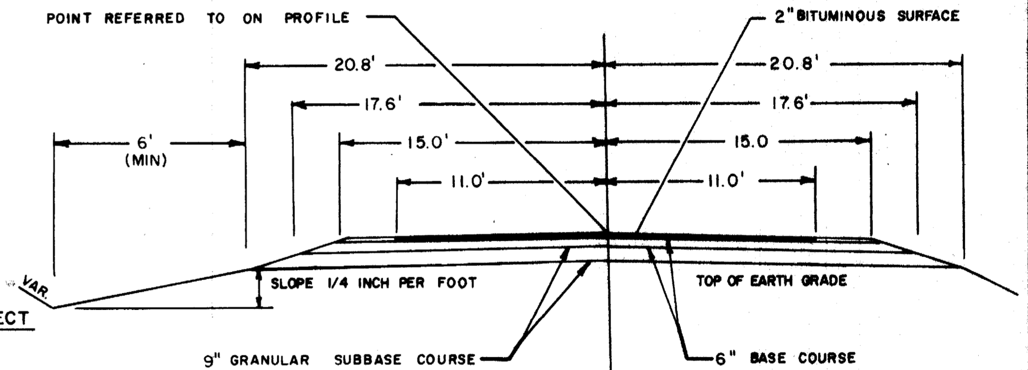
TYPICAL 30' SECTION
